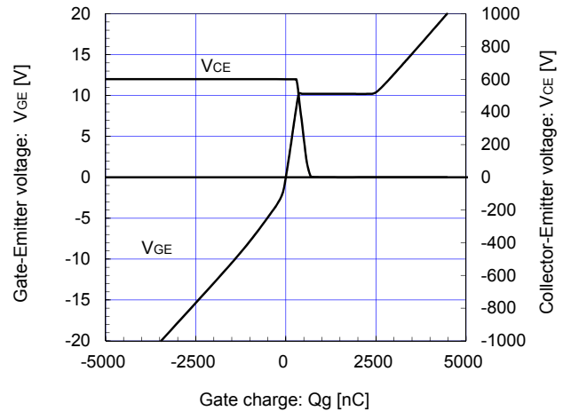
Dynamic Gate Charge (typ.) Vcc=600V, Ic=450A, Tj= 25°C
