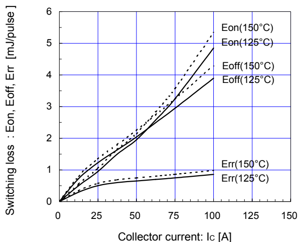
[ Inverter ]
